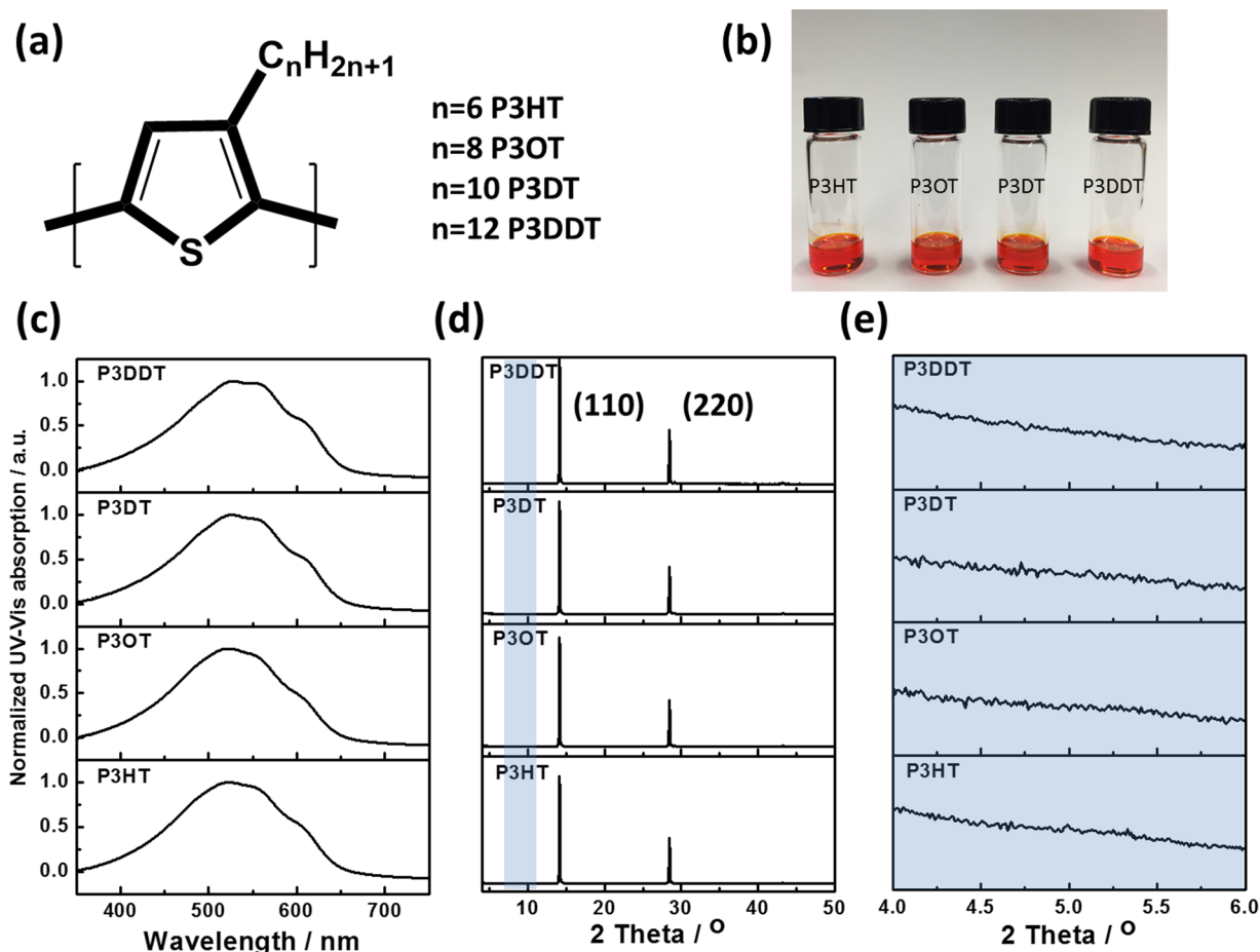
Figure 1. (a) Chemical formula of the PT derivatives used as the HTL material in this study. (b) PT derivatives dissolved in chlorobenzene show identical solution colors. (c) UV-vis spectra of spin-coated PT derivative thin films. (d) X-ray diffraction patterns of fabricated perovskite solar cells without silver electrodes. (e) Zoomed-in X-ray diffraction signals at 2\theta ranging from 4.0^\circ to 6.0^\circ of the corresponding signals shown in (d).
